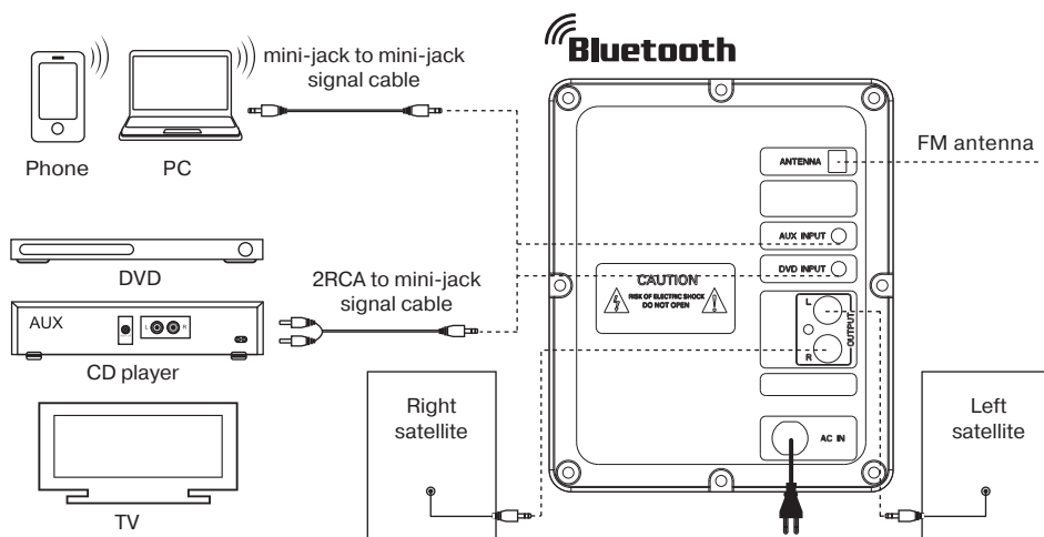
Fig. 4. Connection diagram
